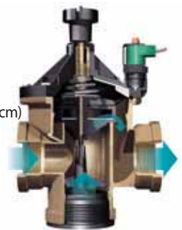
BPES Cutaway
