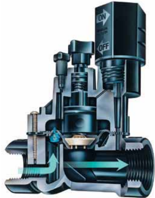
DVF Cutaway
